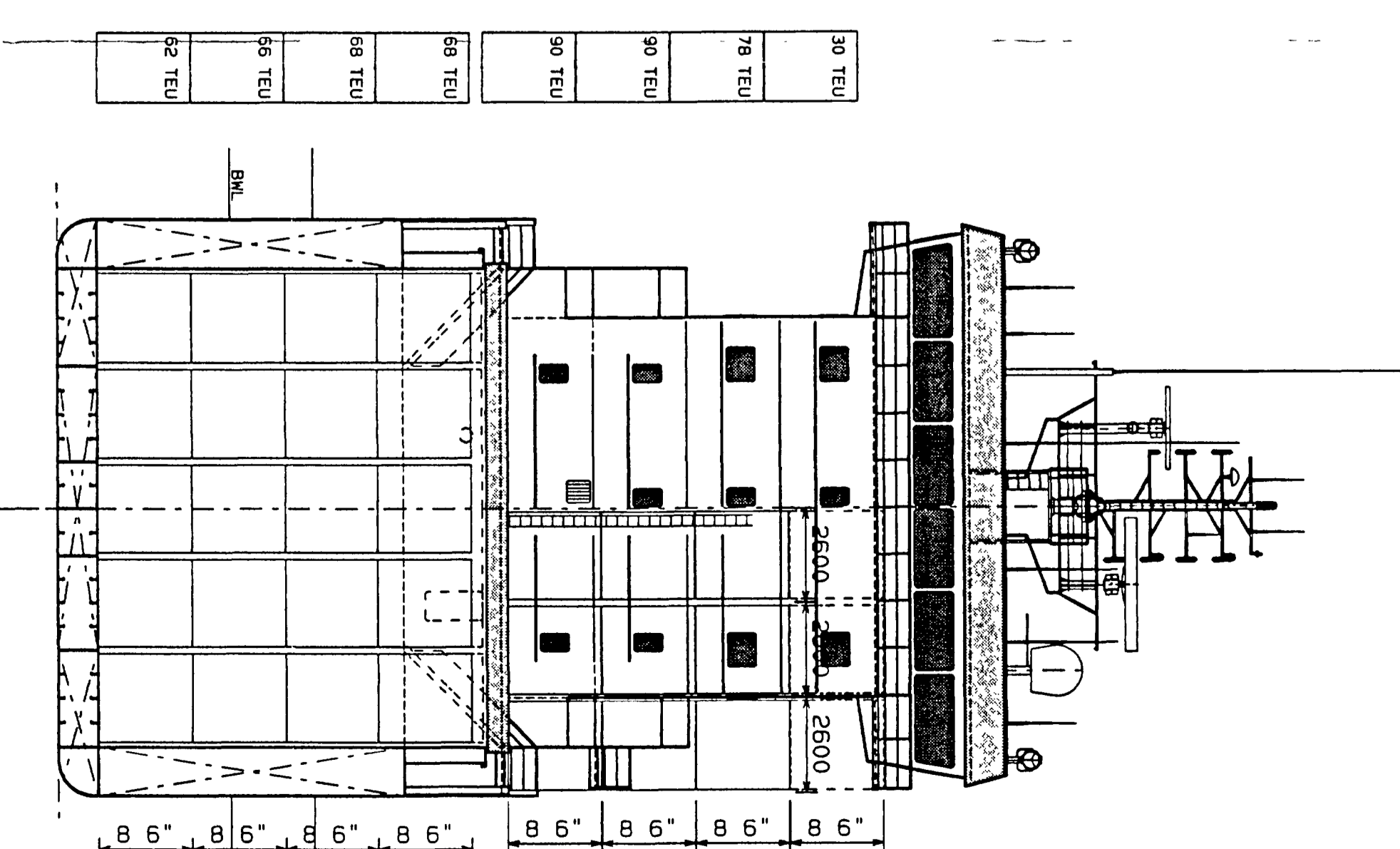
CAPTAINSDACK 20150
