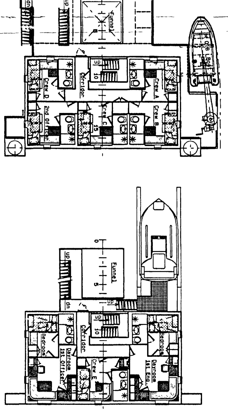
BOATDECK 14950
